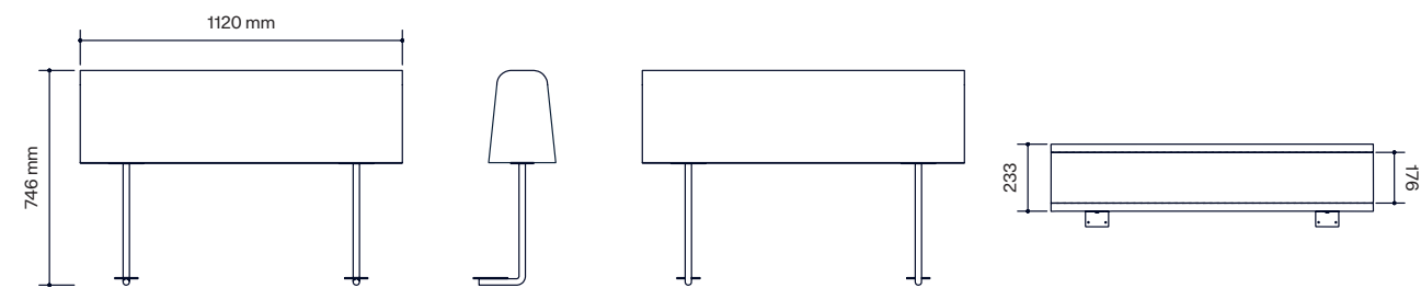
Between backrest
