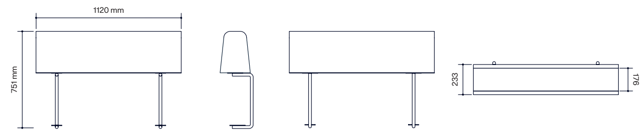
Flush backrest
