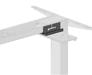
Accessory Bracket 2.0 for beam
